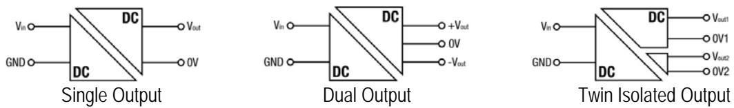
Fig. 2: Standard isolated configurations
