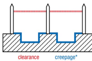
Fig. 9: Clearance and Creepage (* for very small groove dimensions, the creepage is taken to be equal to the clearance – so this simplistic definition must be checked on a case-by-case basis.)
