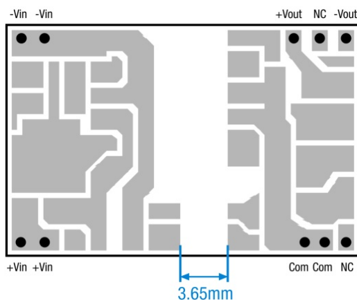
Fig. 10: Example - PCB bottom-side layout showing track separation of 3.65mm. Creepage is the minimum separation measured on both sides of the double-sided PCB.
